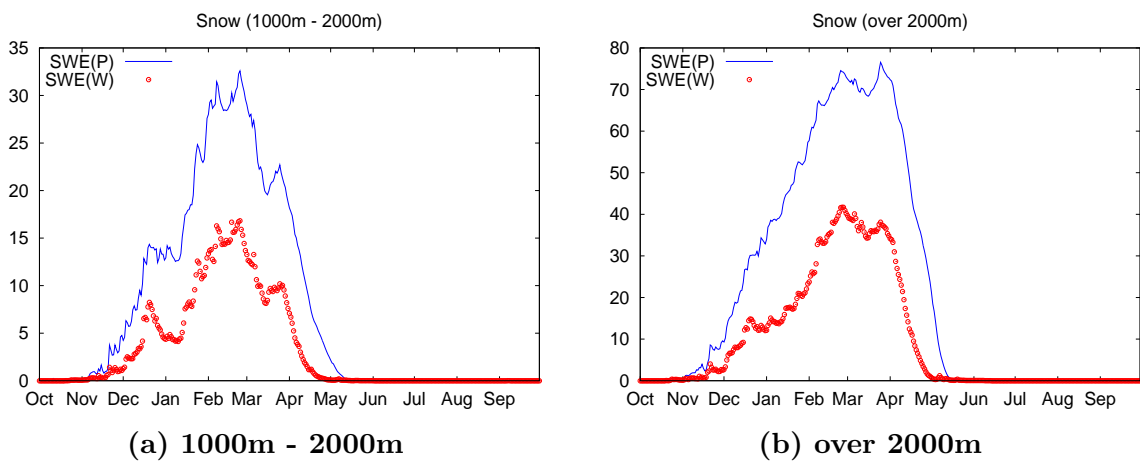
Fig. 6 : Snow water equivalent (daily)
